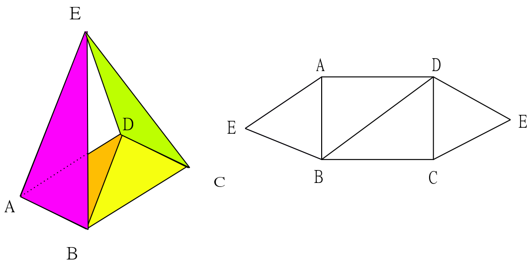
Figure 1: 2-pseudomanifold \mathcal{K}
