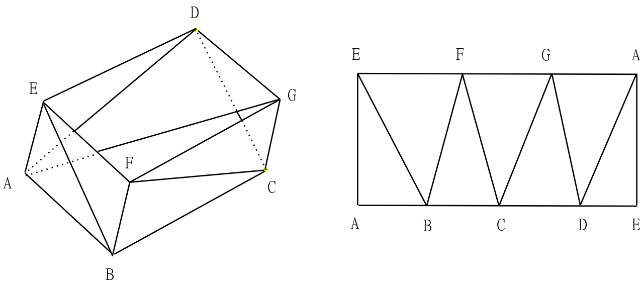
Figure 2: 2-pseudomanifold \mathcal{K} (Möbius band)
