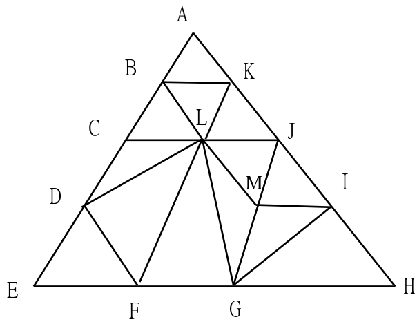
Figure 4: Triangulation T
